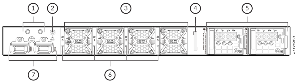
Figure 2: Rear Panel Components of NFX350
