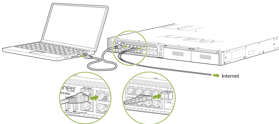
Figure 4: Connecting the Interfaces on an NFX350 Device
