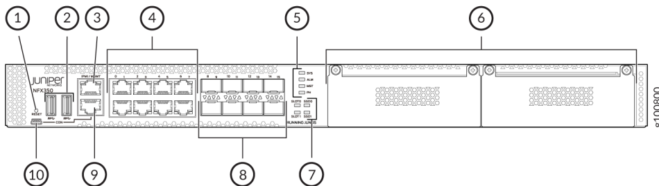
Figure 1: Front Panel Components of NFX350
