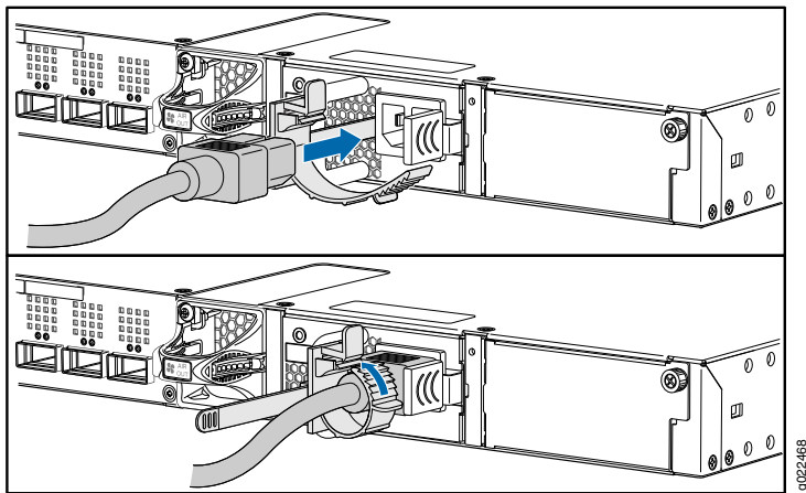
Figure 2: Connecting Power to an EX4300-48MP Switch
