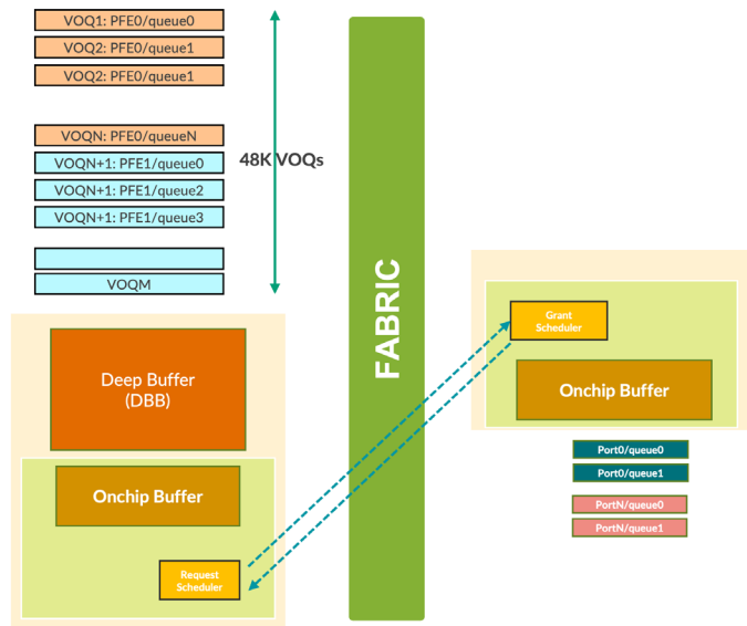
VOQ Architecture
